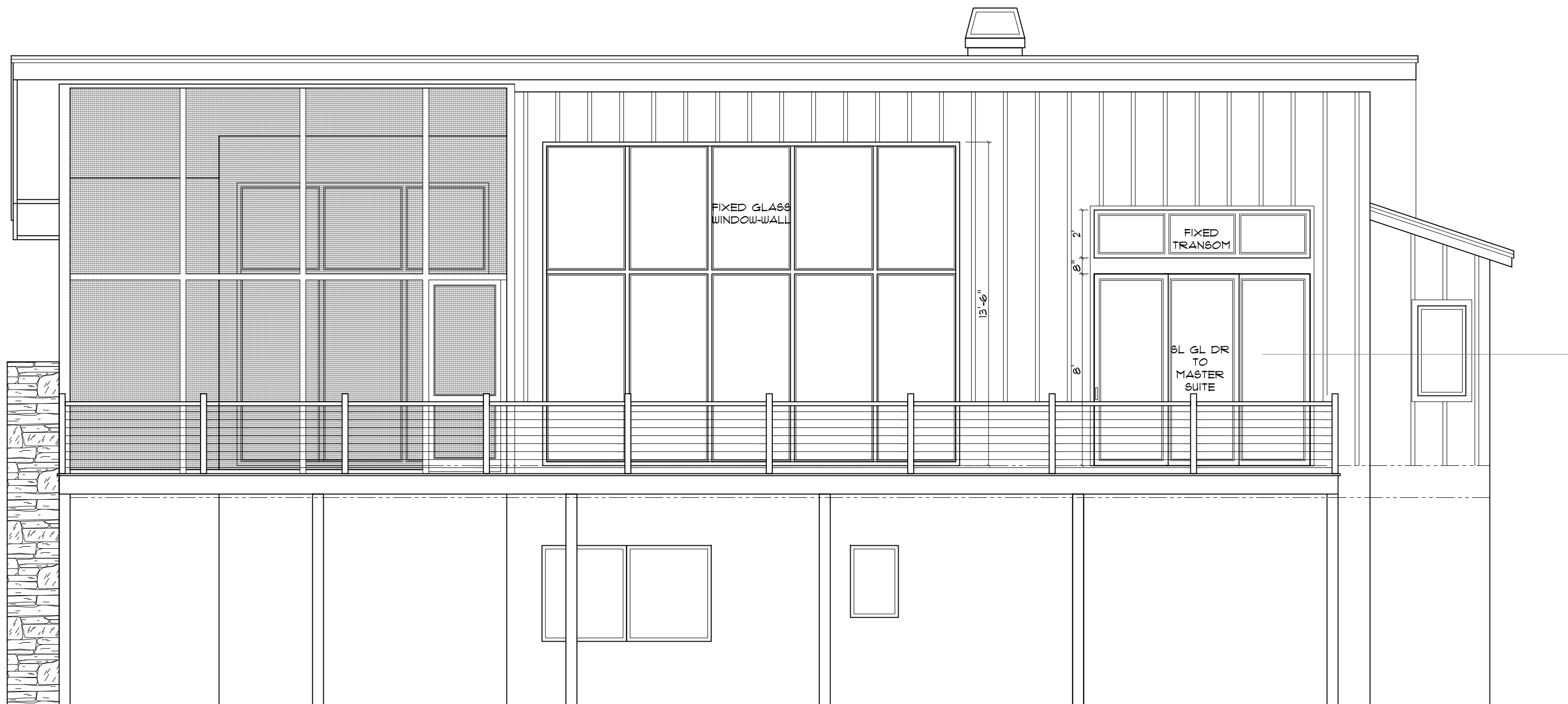
REAR ELEVATION 1/4" = 1'-0"
