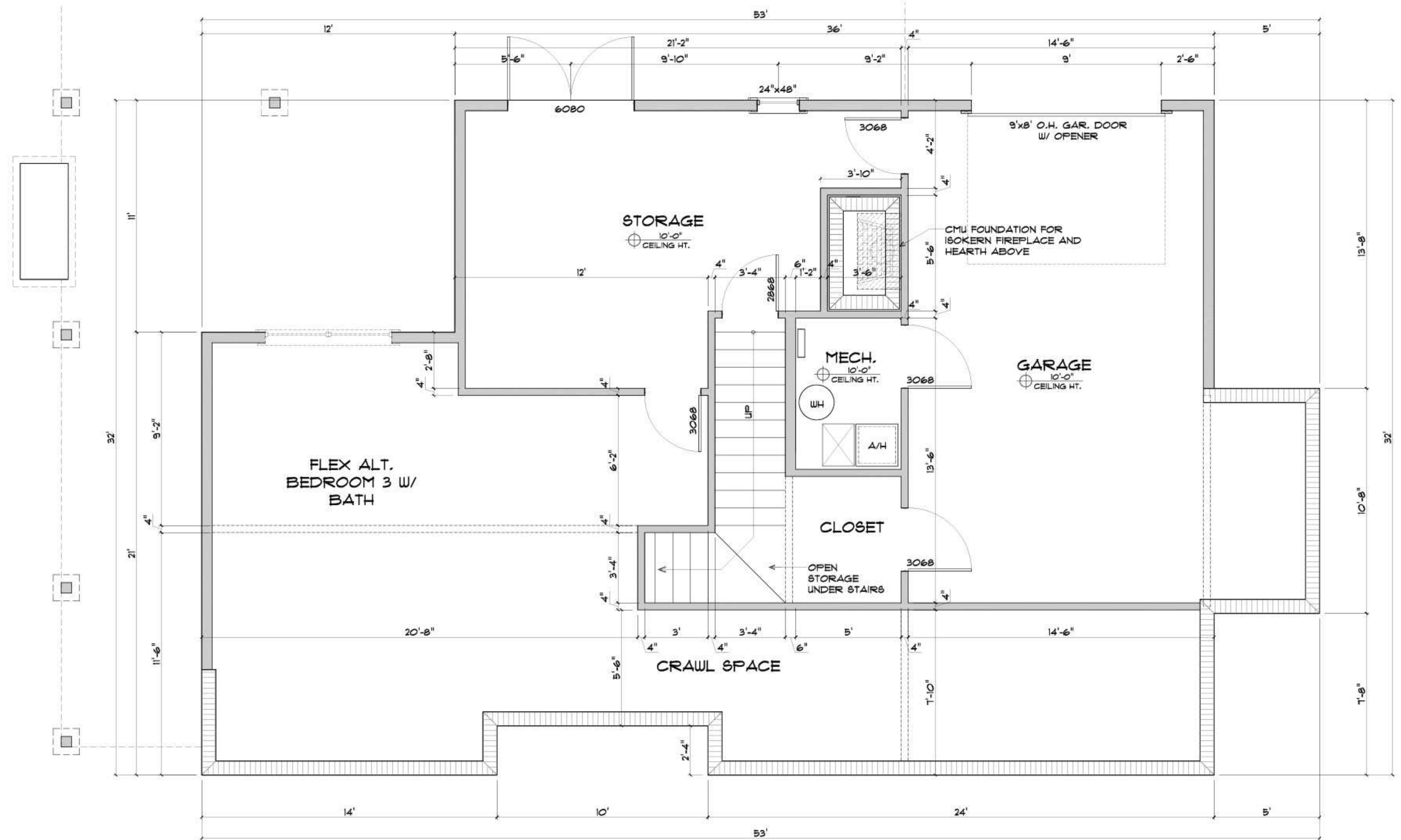
FLOOR PLAN - LOWER LEVEL 1/4" = 1'-0"
