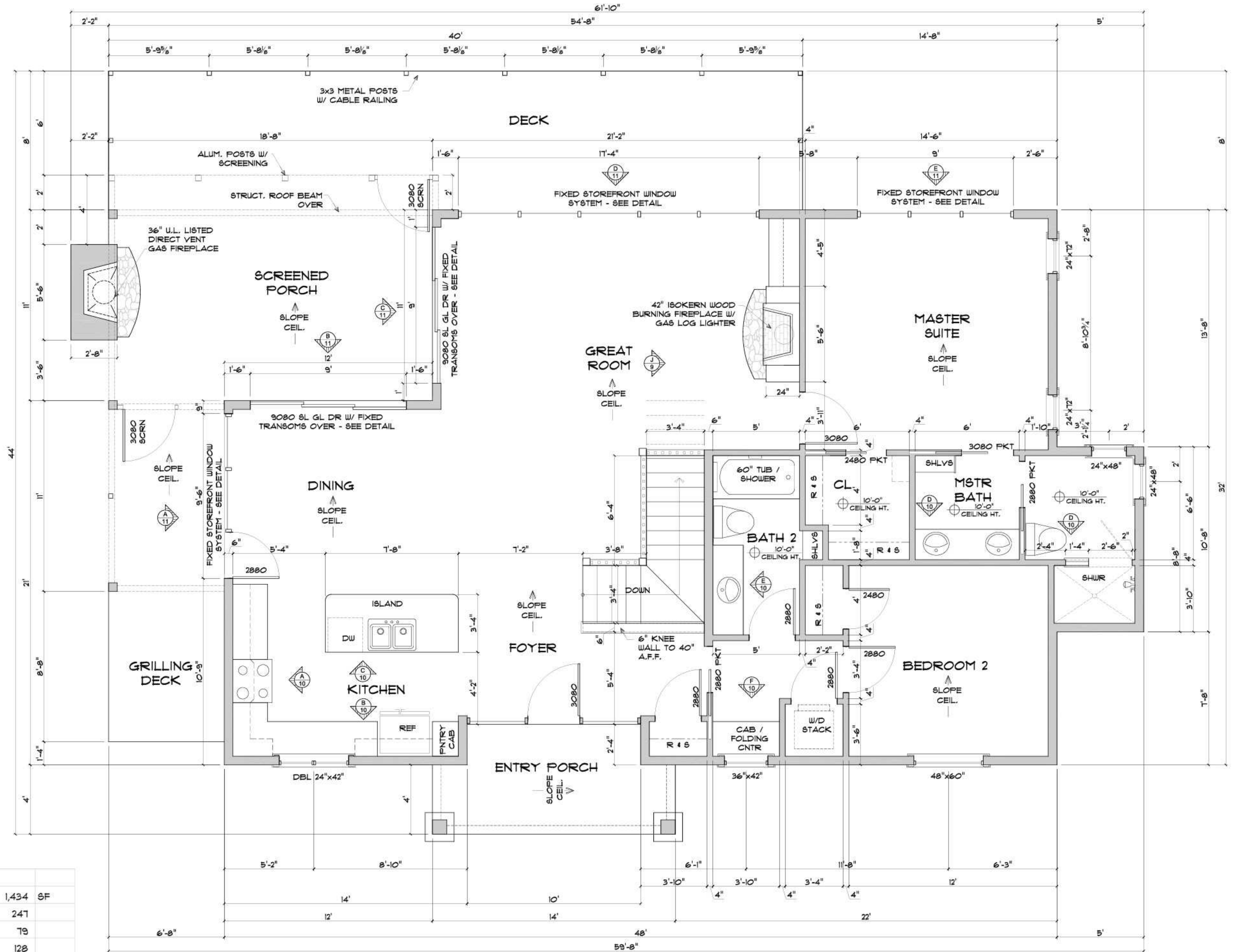
FLOOR PLAN 1/4" = 1'-0"
